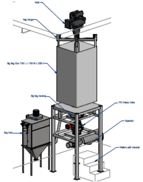
Small Bag Dump Station & Bulk Bag unloading Station with Dust Free Solution
