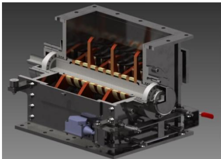
Small Bag Dump Station & Bulk Bag unloading Station with Dust Free Solution
