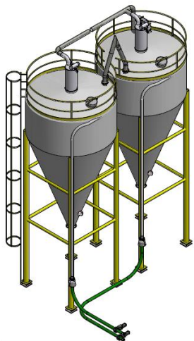
Bulk Truck Loading Station with Silo Weighting System
