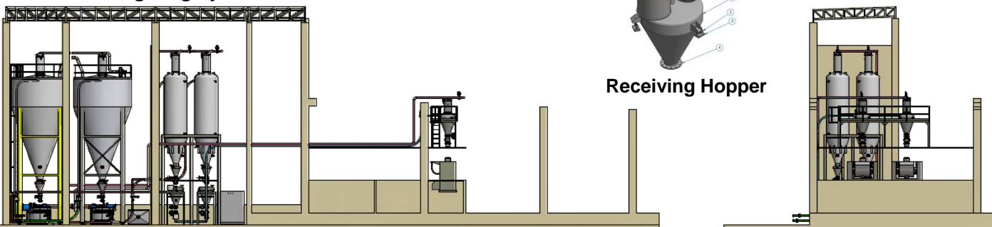
Bulk Truck Loading Station with Silo Weighting System
