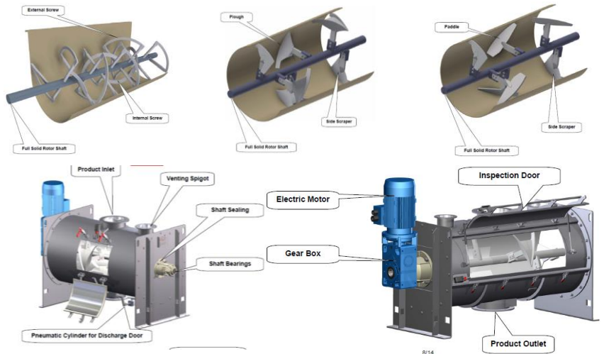
Easy Detachable (Food Grade, Easy Clean) Mixer
