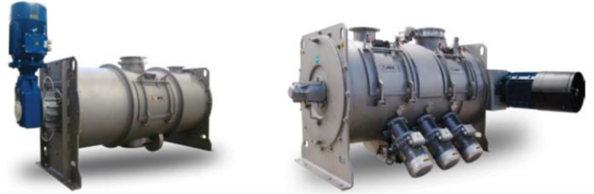
Ploughshare & Mix Paddle Batched Mixer
